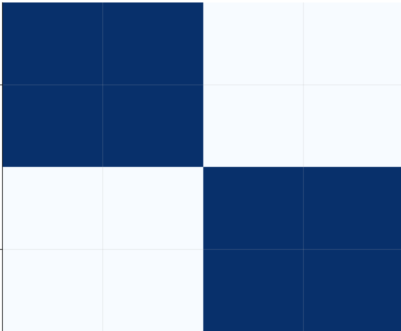
BTCUSDT 15m quantile transition probabilities
